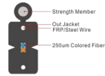
FTTH Self-Support Flat Drop Cable
