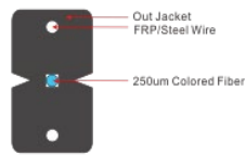
FTTH Flat Cable
